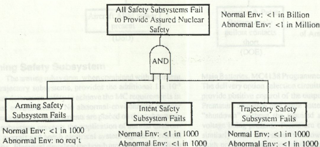
Figure 40. Fault Tree, Loss of Electrical System Safety
